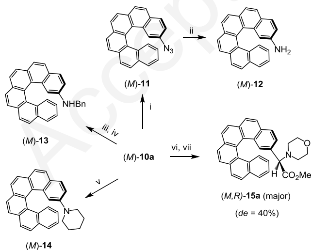
Scheme 3. Synthesis of ( M )-helicenylyl derivatives 12-15 from helicene-boronate ( M )- 10a . Reagents and conditions: i) NaN 3 , CuSO 4 ·5H 2 O, MeOH, reflux, 19h; ii) H 2 (1 atm), 10% Pd/C, EtOAc, rt, 21h, 75% (2 steps); iii) BCl 3 , CH 2 Cl 2 , rt, 3h; iv) PhCH 2 N 3 , CH 2 Cl 2 , rt, 17h, 68% (two steps); v) Cu(OAc) 2 , B(OH) 3 , piperidine, MeCN, 80 °C, 26h, 44%; vi) morpholine, glyoxylic acid monohydrate, 1,1,1,3,3,3-hexafluoro-2-propanol, 60 °C, 48h; vii) (trimethylsilyl)diazomethane in diethyl ether, THF/MeOH, rt, 20h, 84% (two steps).
